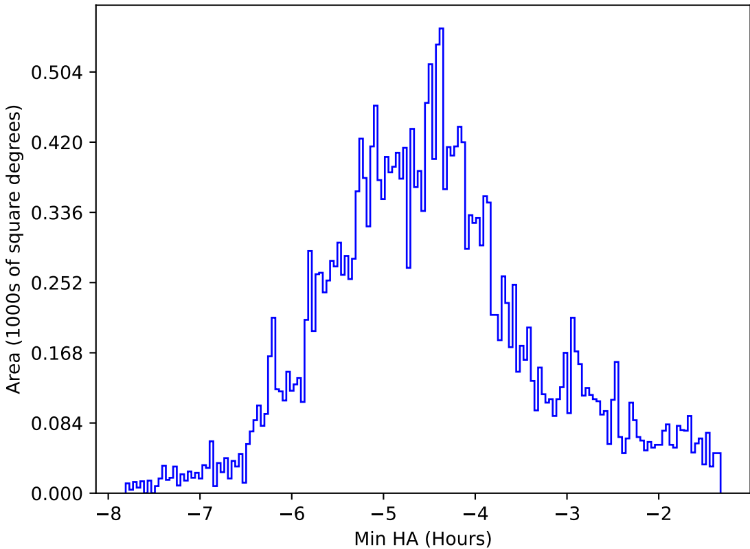
ddf_acor_sf15_lsf30_lsr20_v3.4_10yrs All sky all bands: Min HA
