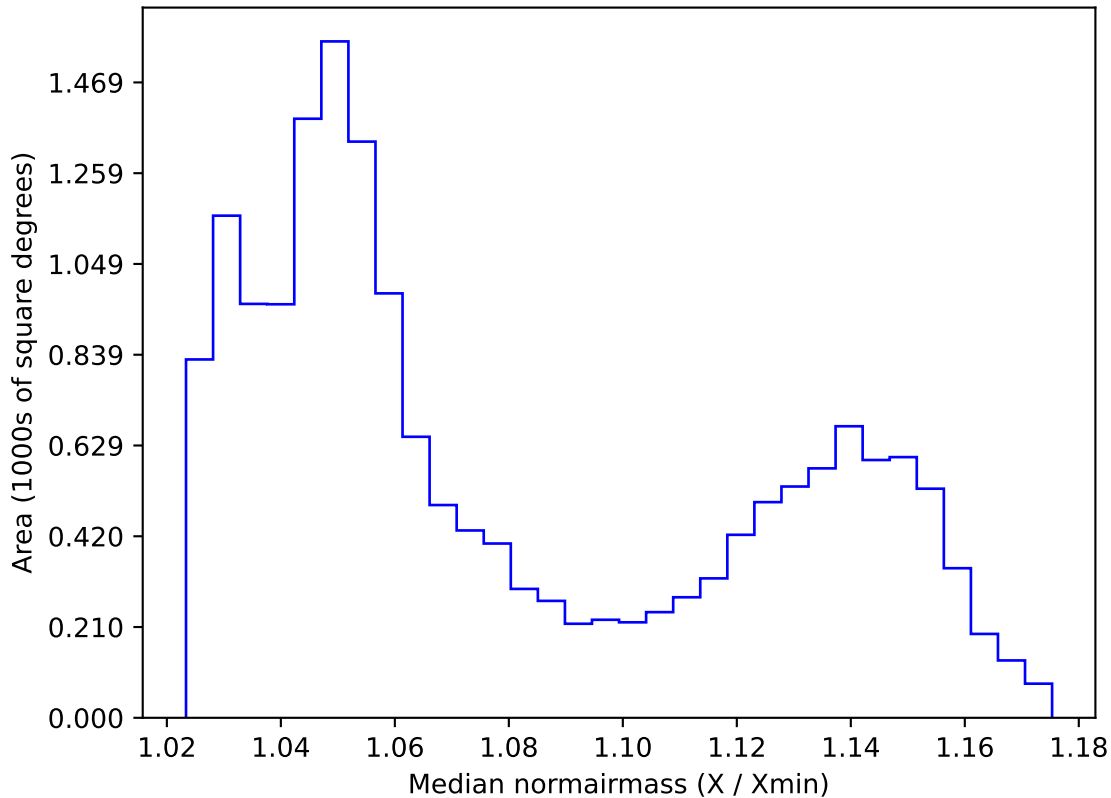
ddf_acor_sf15_lsf30_lsr20_v3.4_10yrs WFD all bands: Median normairmass
