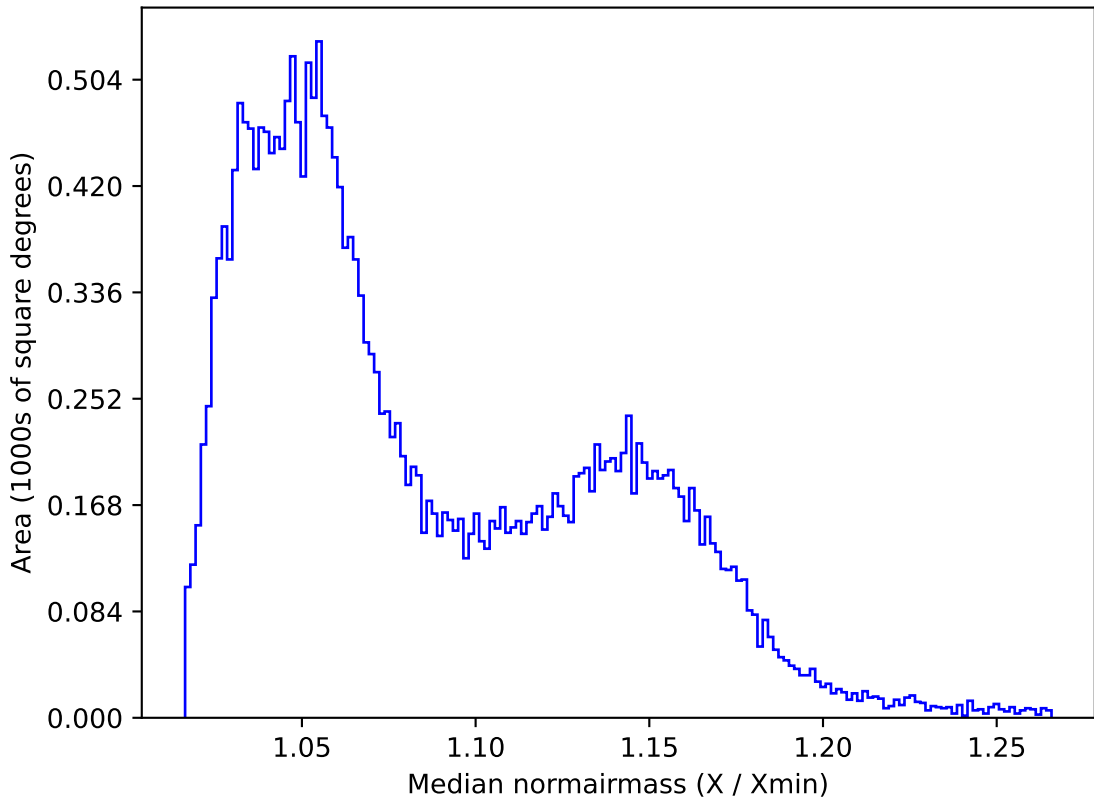
ddf_acor_sf15_ls30_lsr20_v3.4_10yrs All sky z band: Median normairmass
