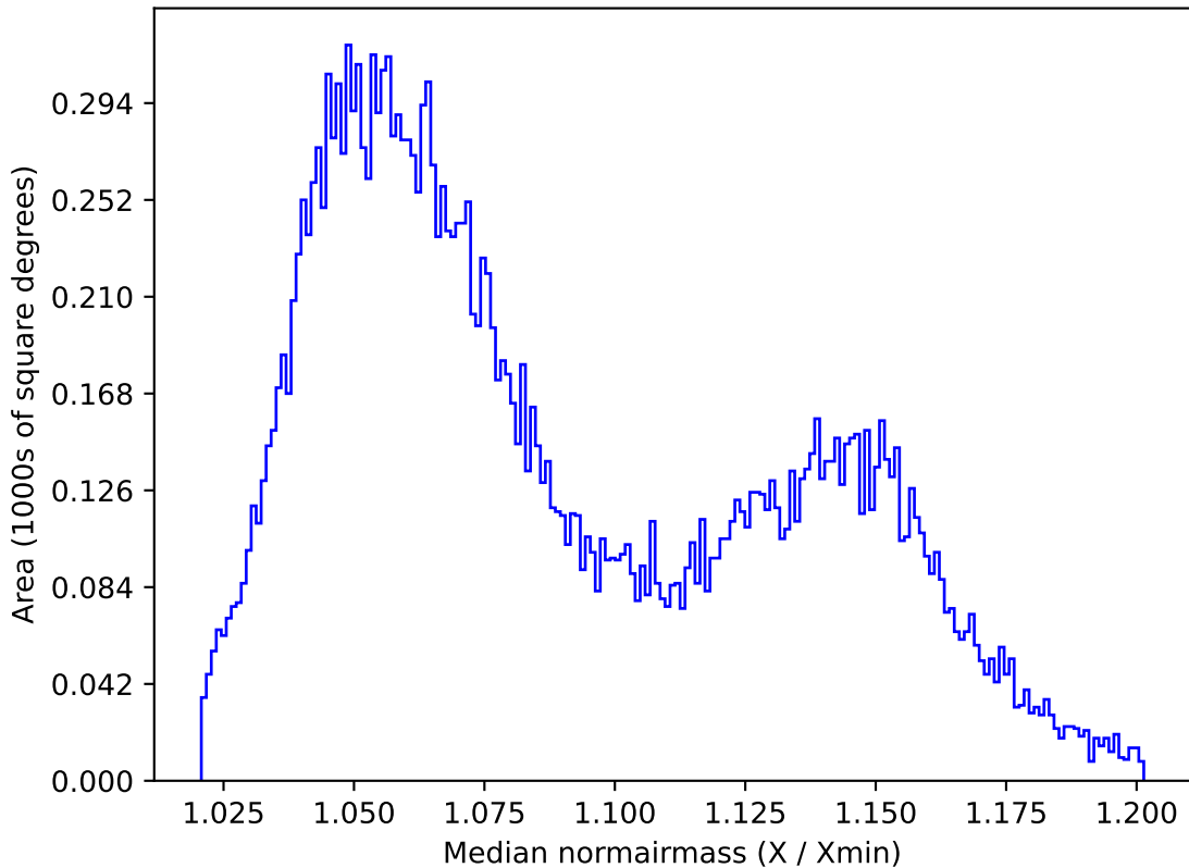
ddf_acor_sf15_ls30_lsr20_v3.4_10yrs All sky y band: Median normairmass
