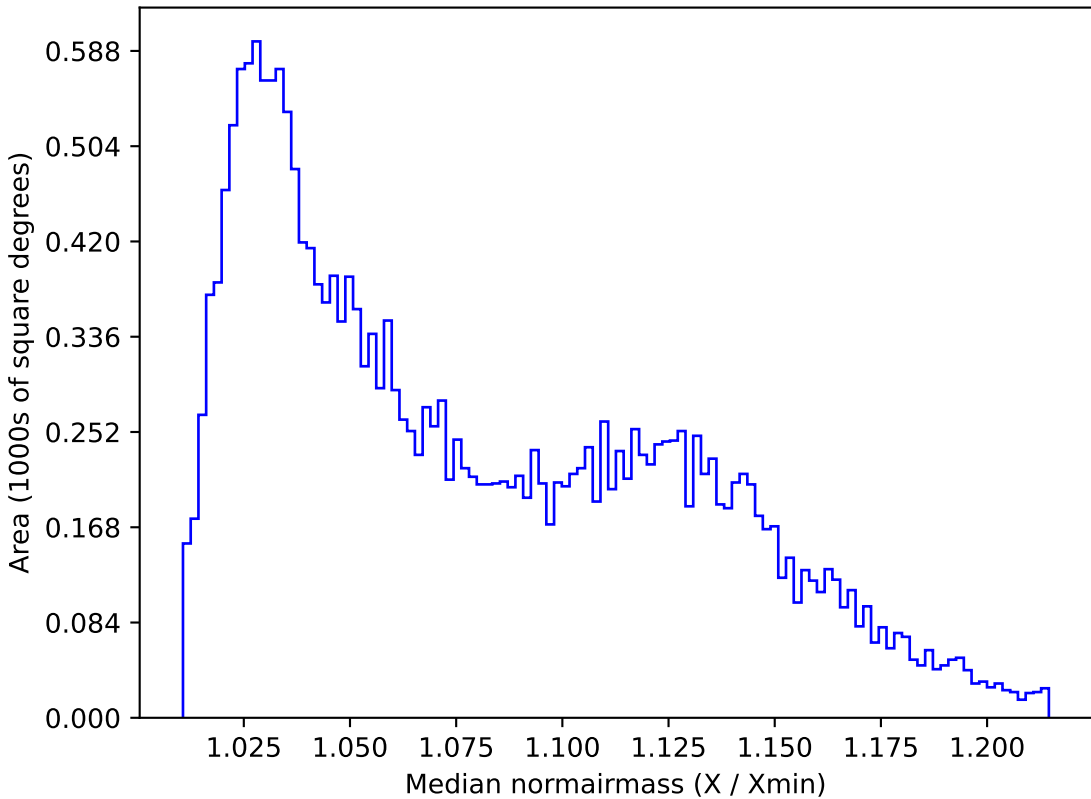
ddf_acor_sf15_lsf30_lsr20_v3.4_10yrs All sky u band: Median normairmass
