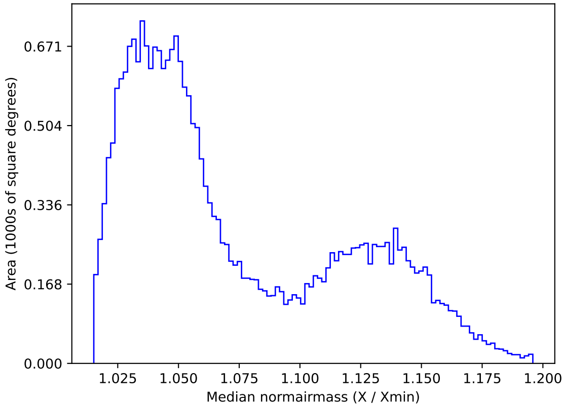
ddf_acor_sf15_lsf30_lsr20_v3.4_10yrs All sky i band: Median normairmass
