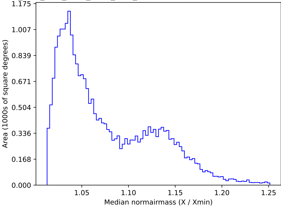
ddf_acor_sf15_lsf30_lsr20_v3.4_10yrs All sky g band: Median normairmass
