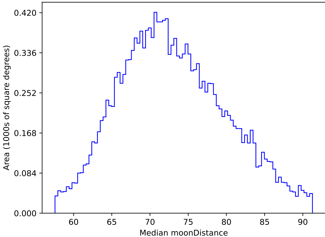
ddf_acor_sf15_lsf30_lsr20_v3.4_10yrs WFD z band: Median moonDistance
