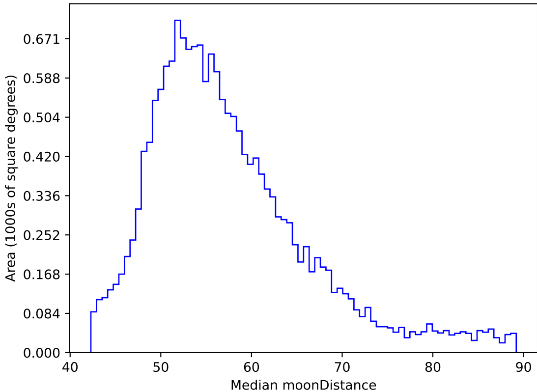
ddf_acor_sf15_lsf30_lsr20_v3.4_10yrs WFD y band: Median moonDistance
