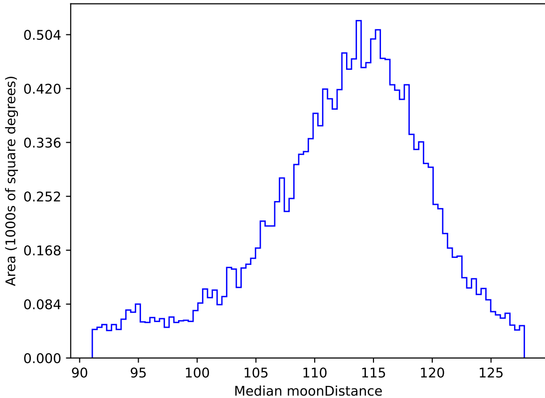
ddf_acor_sf15_lsf30_lsr20_v3.4_10yrs WFD r band: Median moonDistance
