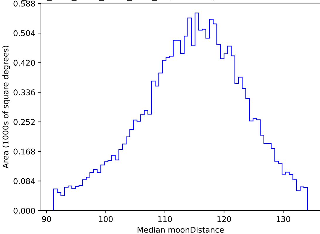
ddf_acor_sf15_lsf30_lsr20_v3.4_10yrs WFD g band: Median moonDistance
