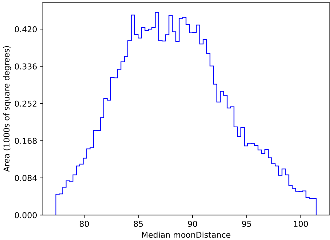
ddf_acor_sf15_lsf30_lsr20_v3.4_10yrs WFD all bands: Median moonDistance
