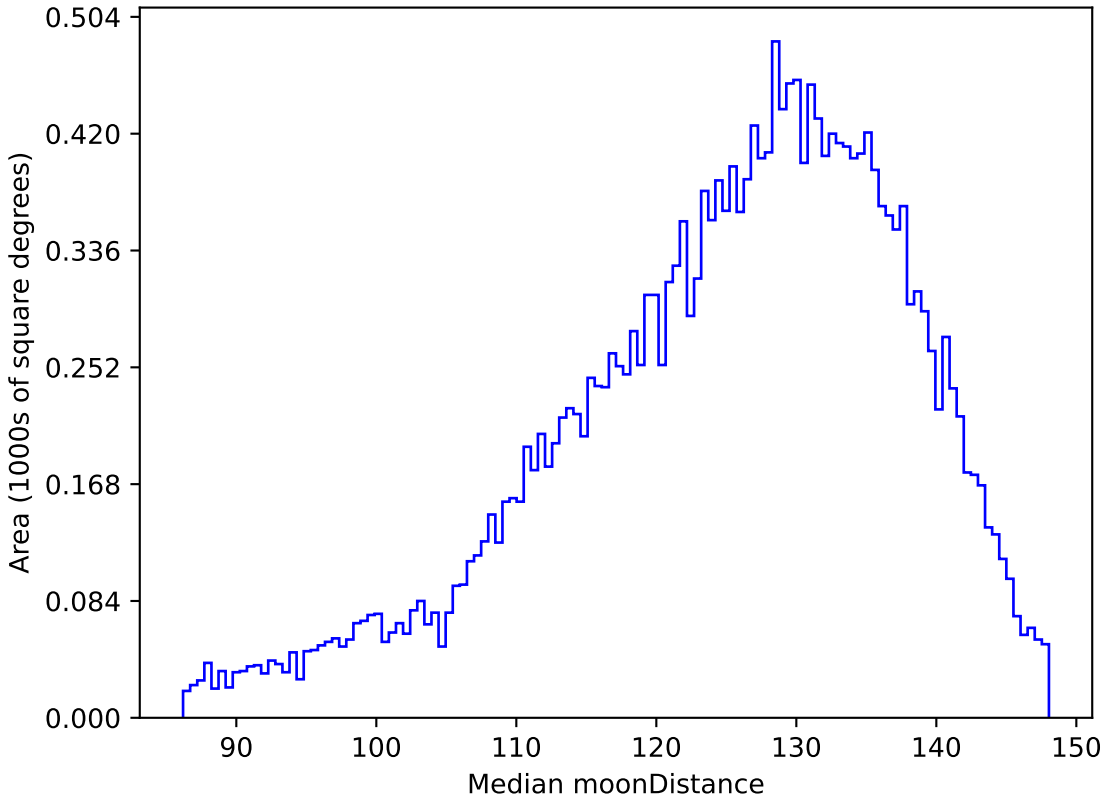
ddf_acor_sf15_lsf30_lsr20_v3.4_10yrs All sky u band: Median moonDistance
