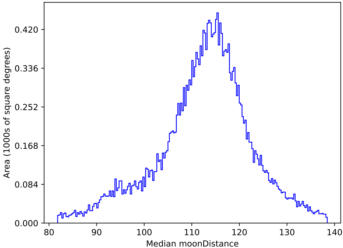
ddf_acor_sf15_lsf30_lsr20_v3.4_10yrs All sky r band: Median moonDistance
