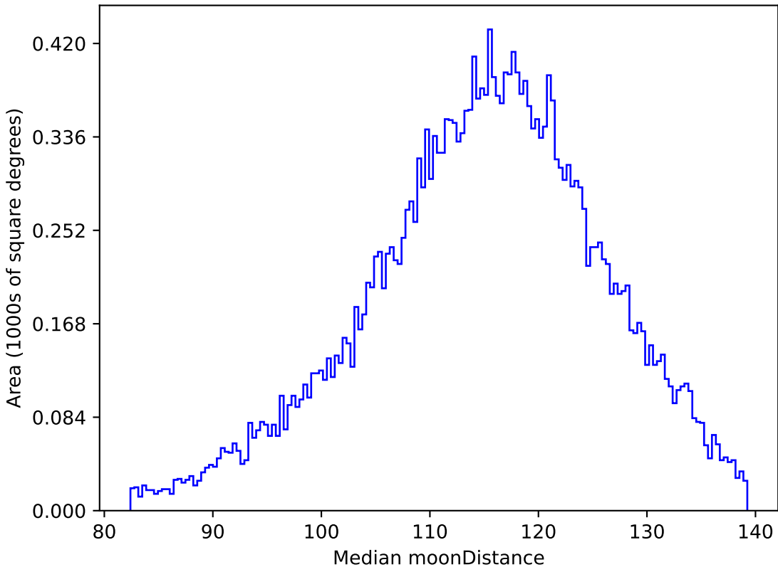
ddf_acor_sf15_lsf30_lsr20_v3.4_10yrs All sky g band: Median moonDistance
