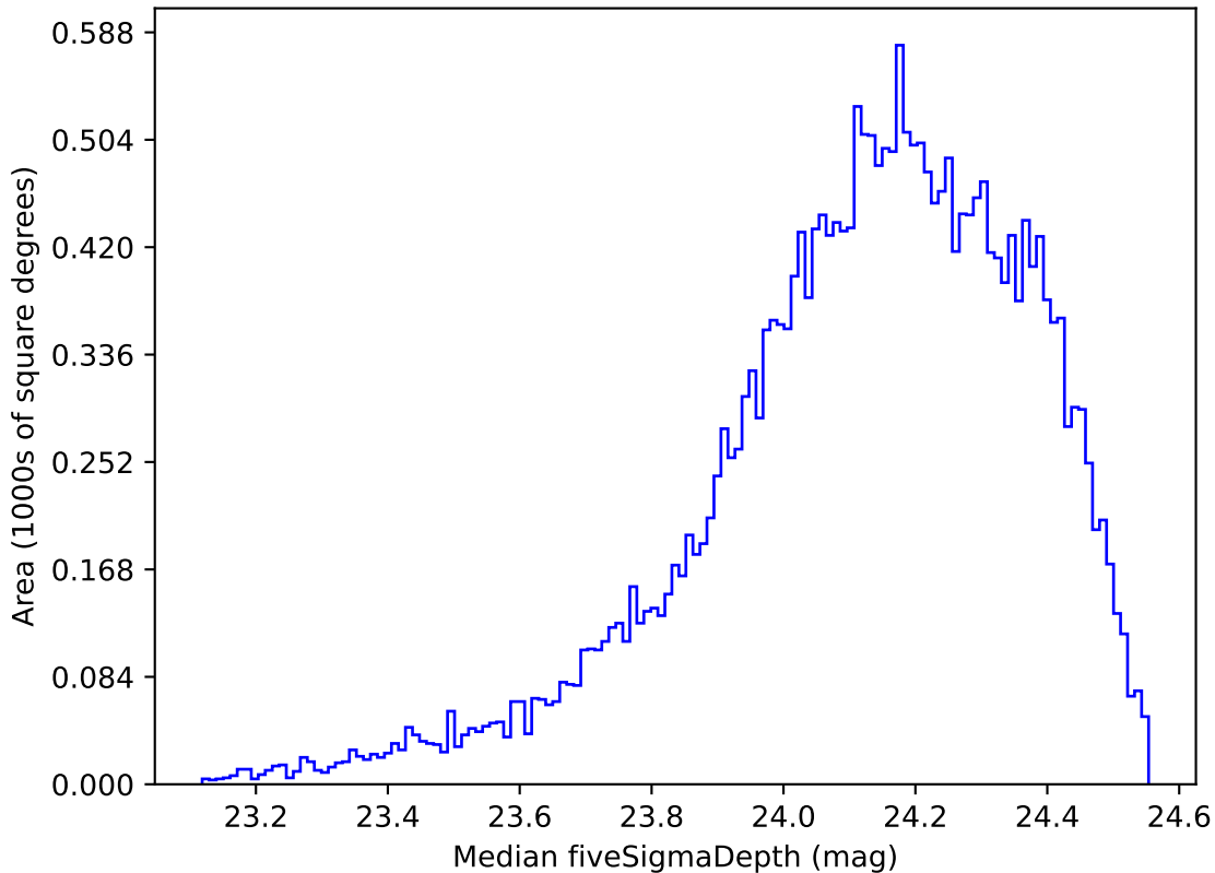
ddf_acor_sf15_lsf30_lsr20_v3.4_10yrs Yr 1 r band: Median fiveSigmaDepth
