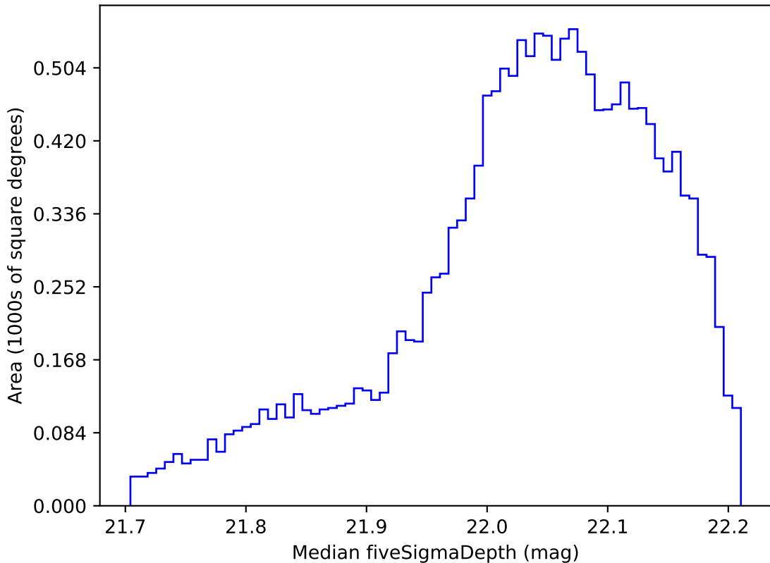
ddf_acor_sf15_lsf30_lsr20_v3.4_10yrs WFD y band: Median fiveSigmaDepth
