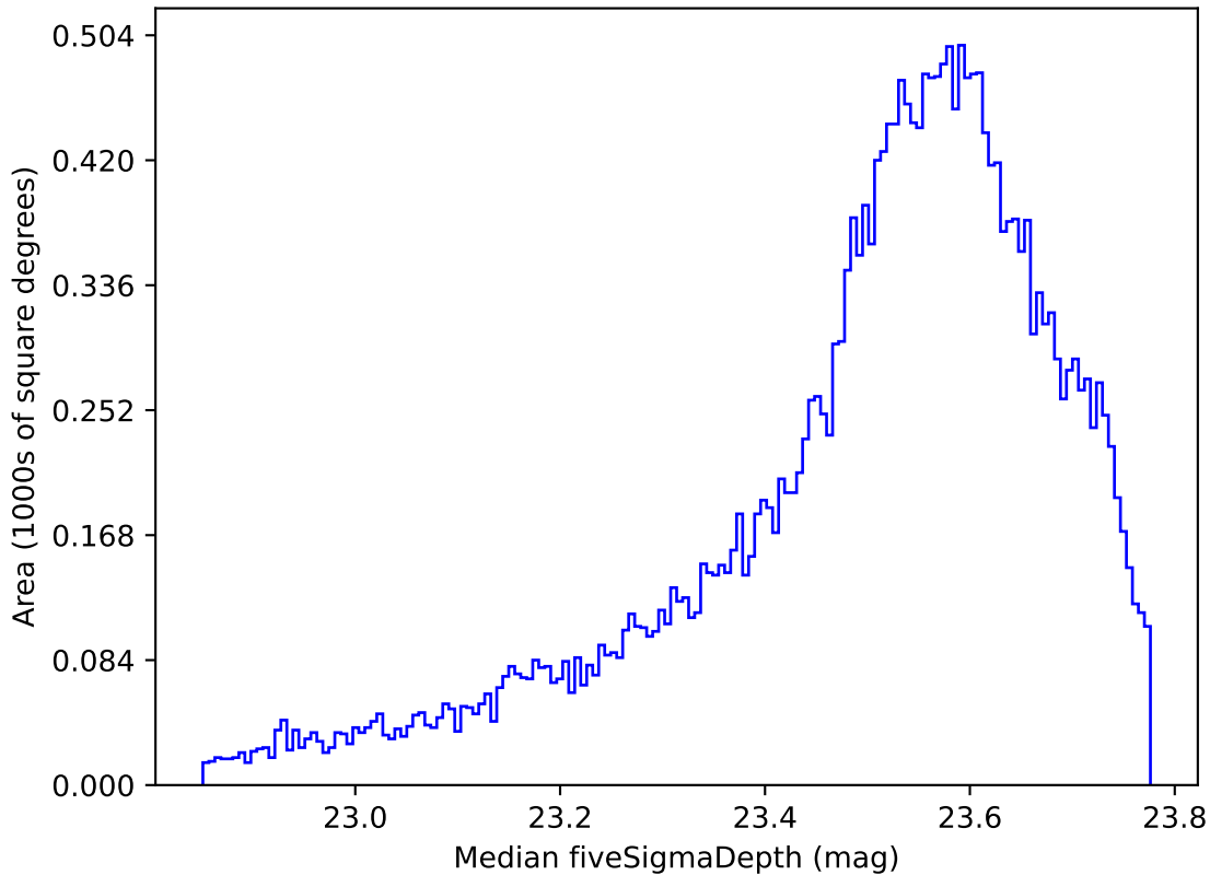
ddf_acor_sf15_lsf30_lsr20_v3.4_10yrs All sky i band: Median fiveSigmaDepth
