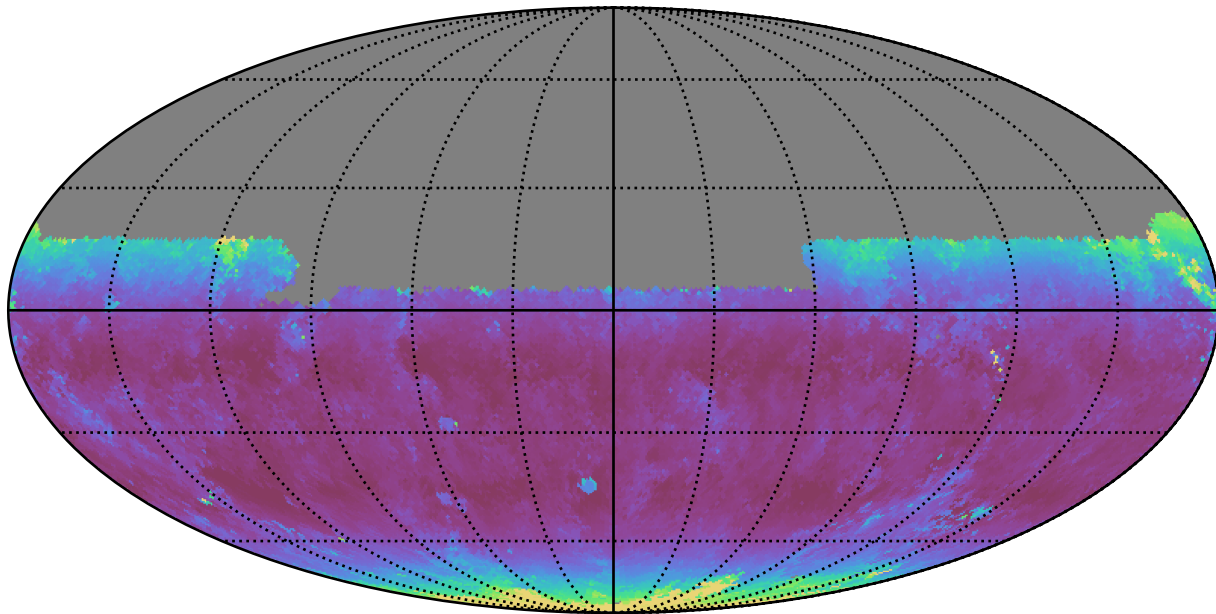
ddf_acor_sf15_lsf30_lsr20_v3.4_10yrs Yr 1 y band: Median airmass
