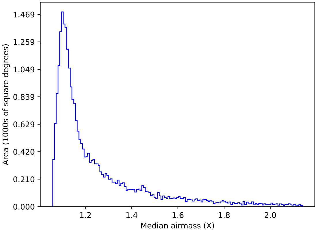
ddf_acor_sf15_lsf30_lsr20_v3.4_10yrs Yr 1 r band: Median airmass
