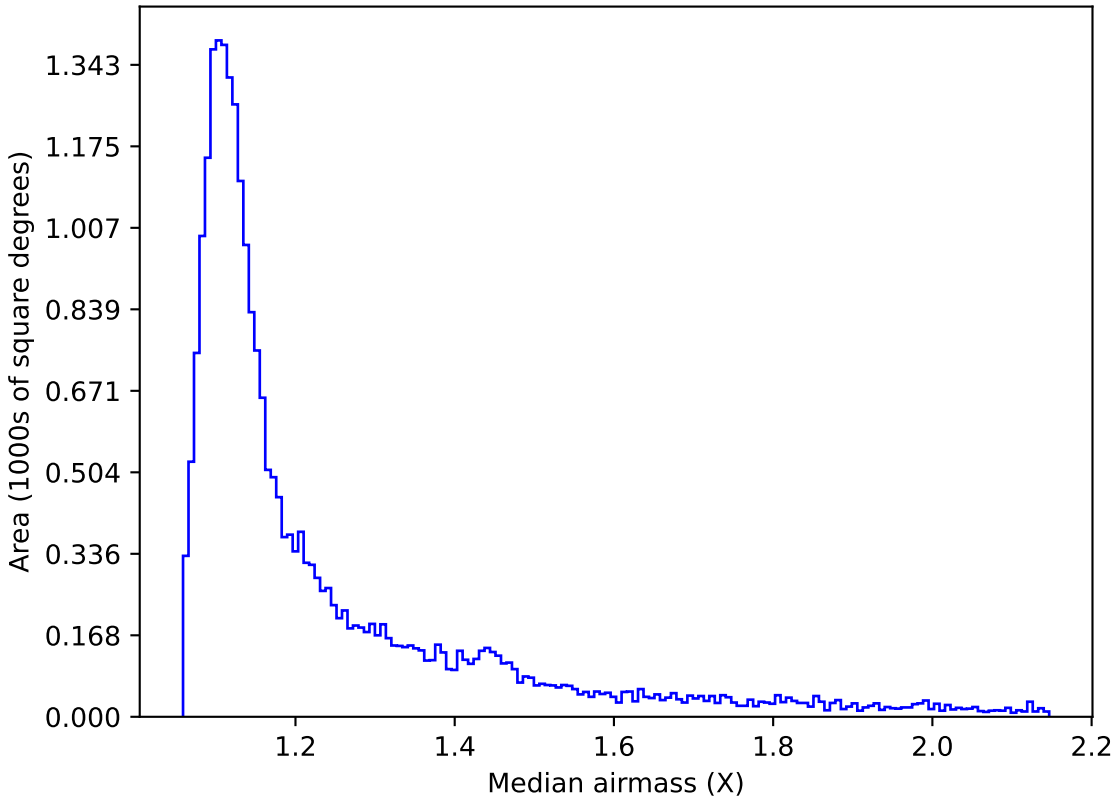
ddf_acor_sf15_lsf30_lsr20_v3.4_10yrs Yr 1 i band: Median airmass
