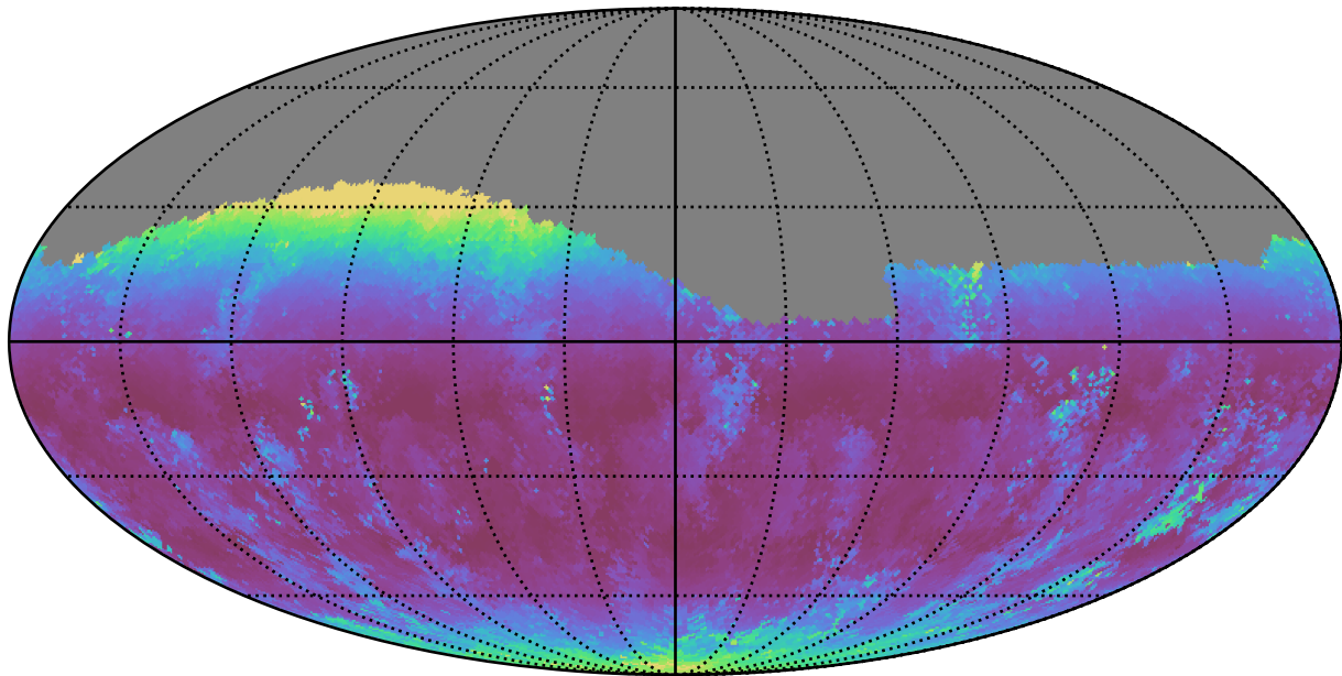
ddf_acor_sf15_lsf30_lsr20_v3.4_10yrs Yr 1 g band: Median airmass
