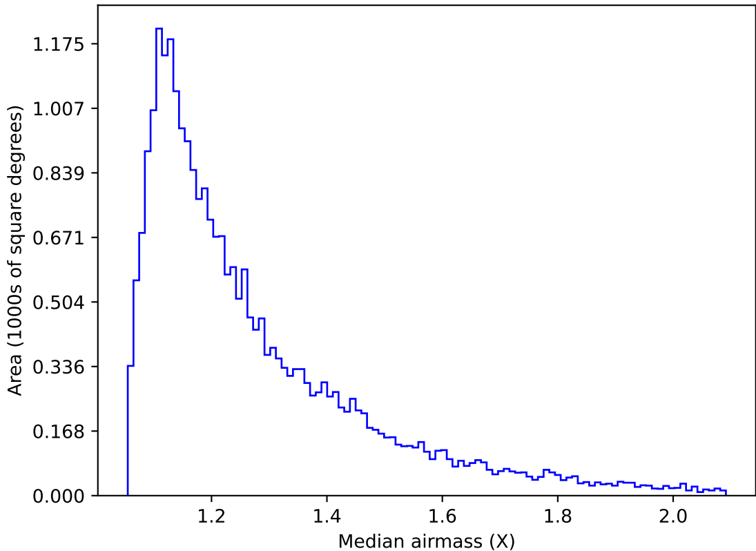
ddf_acor_sf15_lsf30_lsr20_v3.4_10yrs Yr 1 g band: Median airmass
