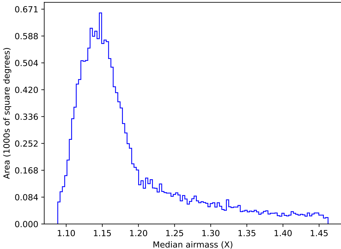
ddf_acor_sf15_lsf30_lsr20_v3.4_10yrs WFD z band: Median airmass
