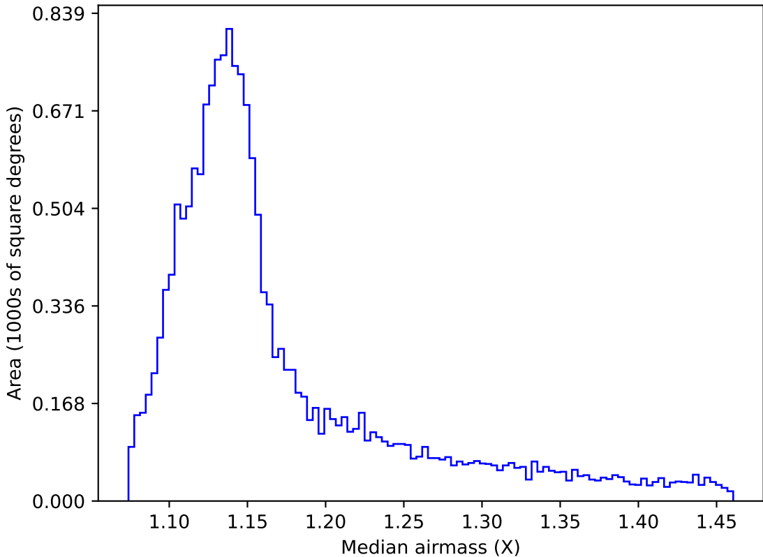
ddf_acor_sf15_lsf30_lsr20_v3.4_10yrs WFD r band: Median airmass
