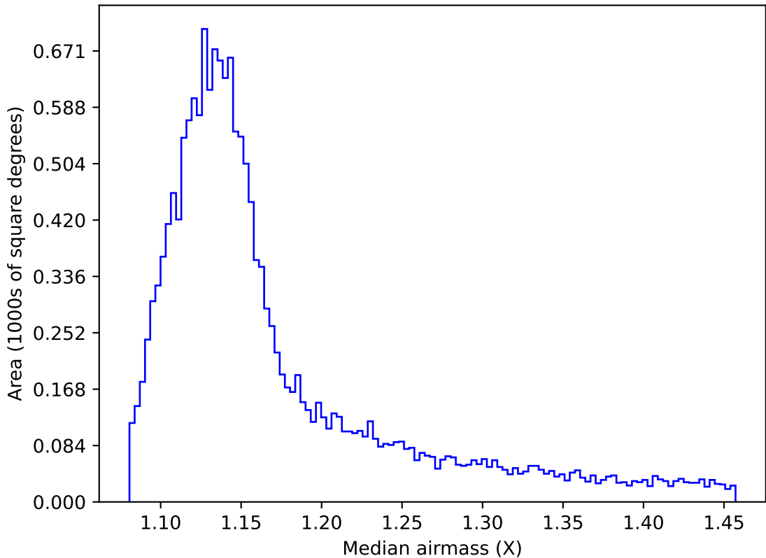
ddf_acor_sf15_lsf30_lsr20_v3.4_10yrs WFD i band: Median airmass
