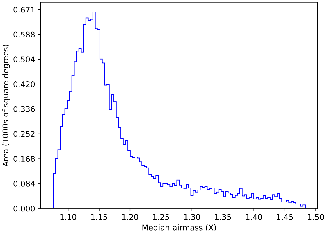
ddf_acor_sf15_lsf30_lsr20_v3.4_10yrs WFD g band: Median airmass
