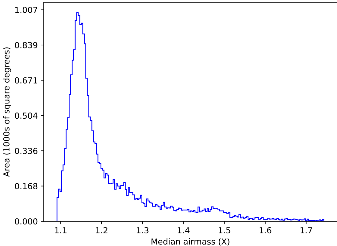
ddf_acor_sf15_lsf30_lsr20_v3.4_10yrs All sky y band: Median airmass
