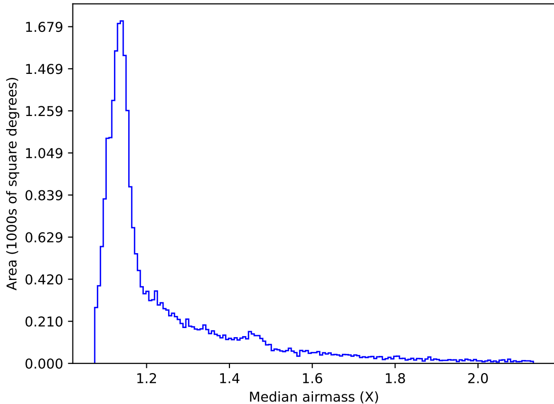
ddf_acor_sf15_lsf30_lsr20_v3.4_10yrs All sky r band: Median airmass
