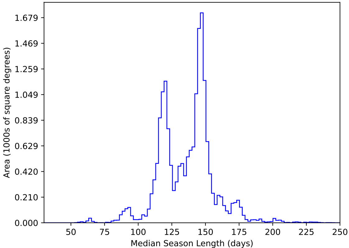
ddf_acor_sf15_lsf30_lsr20_v3.4_10yrs WFD y band: Median Season Length
