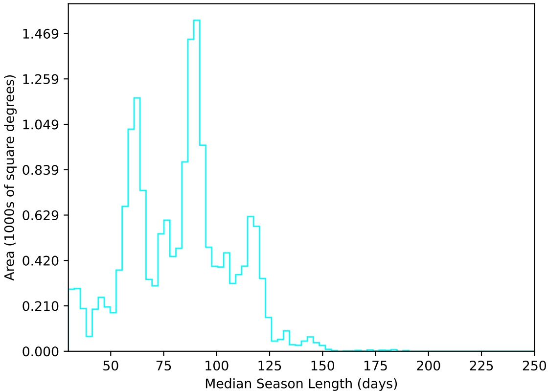
ddf_acor_sf15_ls30_lsr20_v3.4_10yrs WFD u band: Median Season Length
