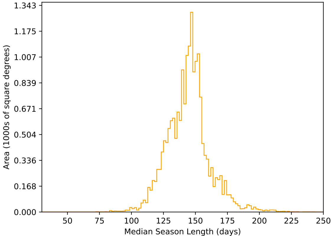
ddf_acor_sf15_lsf30_lsr20_v3.4_10yrs WFD r band: Median Season Length
