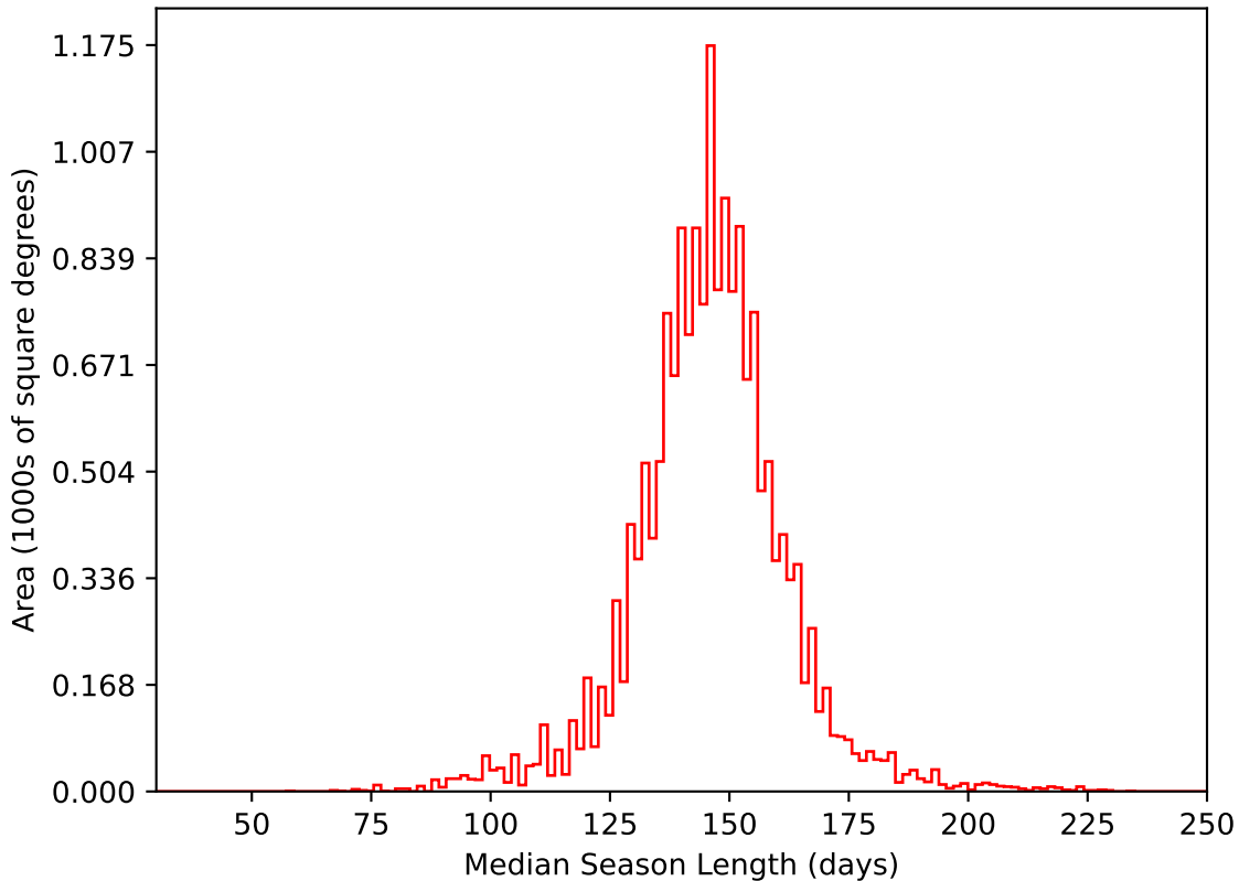
ddf_acor_sf15_lsf30_lsr20_v3.4_10yrs WFD i band: Median Season Length
