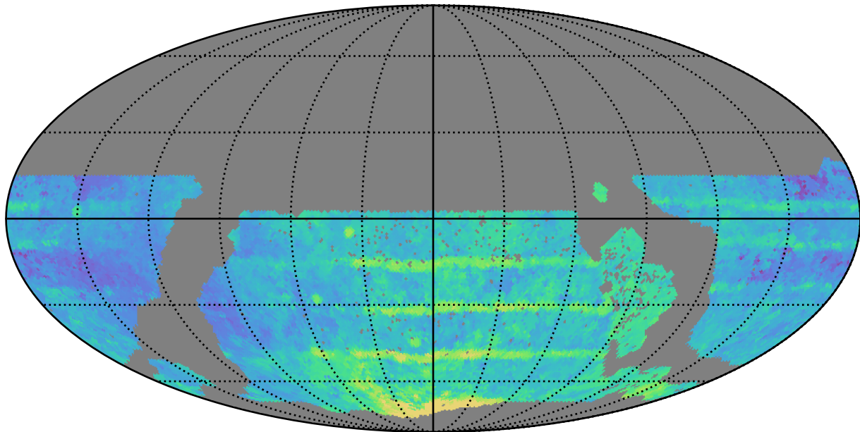
ddf_acor_sf15_lsf30_lsr20_v3.4_10yrs WFD all bands: Median Season Length
