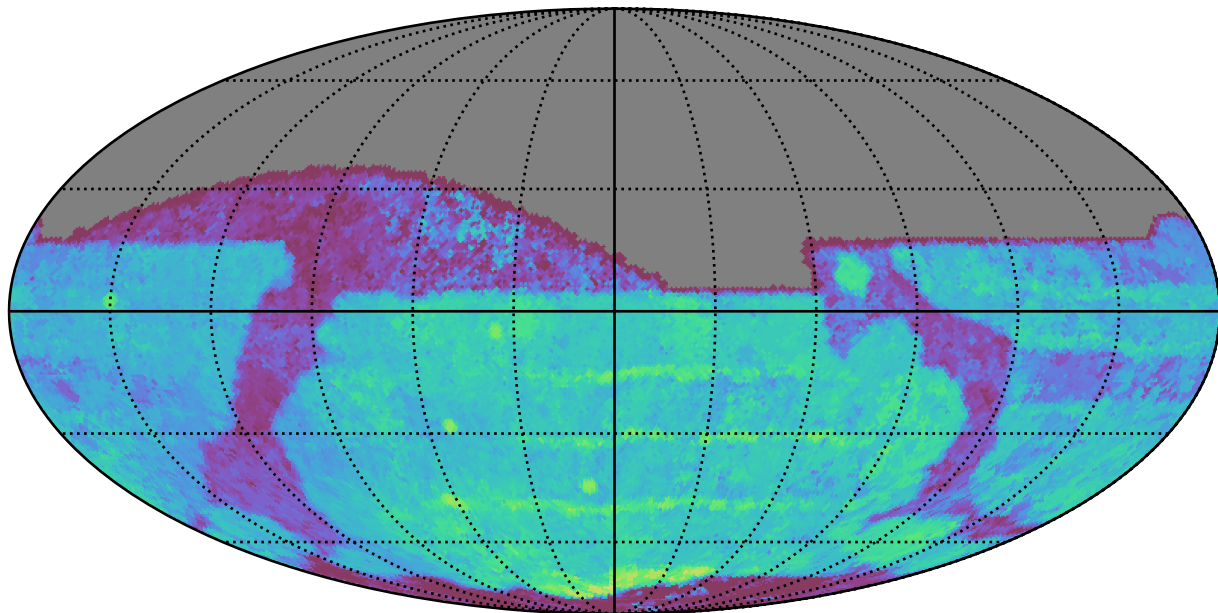
ddf_acor_sf15_lsf30_lsr20_v3.4_10yrs All sky z band: Median Season Length
