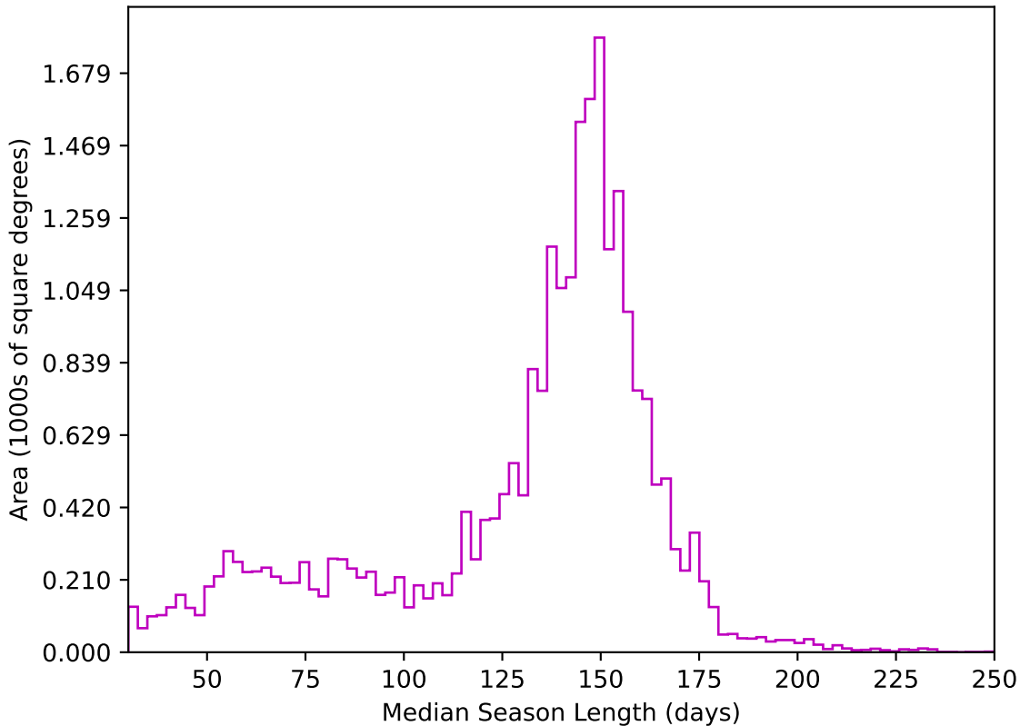
ddf_acor_sf15_lsf30_lsr20_v3.4_10yrs All sky z band: Median Season Length
