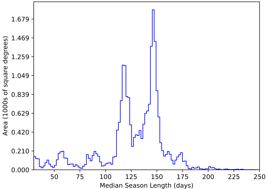
ddf_acor_sf15_lsf30_lsr20_v3.4_10yrs All sky y band: Median Season Length
