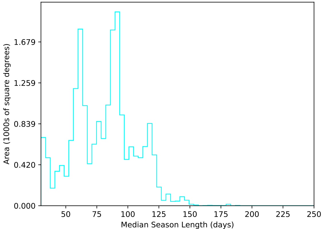
ddf_acor_sf15_lsf30_lsr20_v3.4_10yrs All sky u band: Median Season Length
