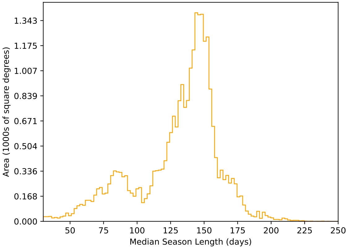
ddf_acor_sf15_lsf30_lsr20_v3.4_10yrs All sky r band: Median Season Length
