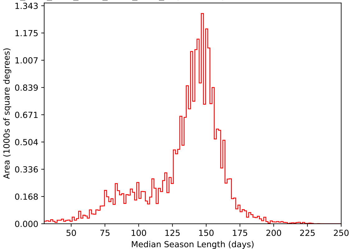
ddf_acor_sf15_lsf30_lsr20_v3.4_10yrs All sky i band: Median Season Length
