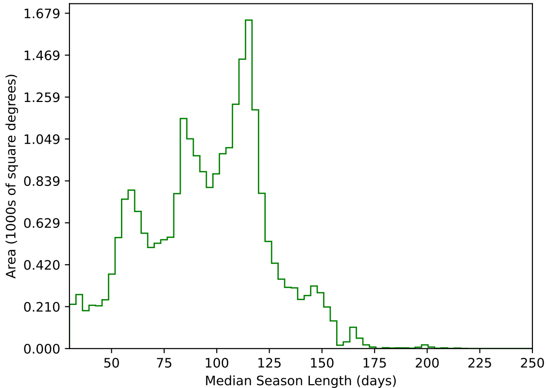
ddf_acor_sf15_lsf30_lsr20_v3.4_10yrs All sky g band: Median Season Length
