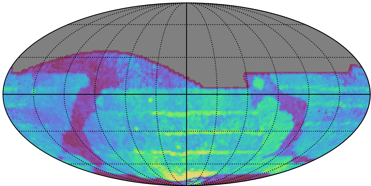
ddf_acor_sf15_lsf30_lsr20_v3.4_10yrs All sky all bands: Median Season Length
