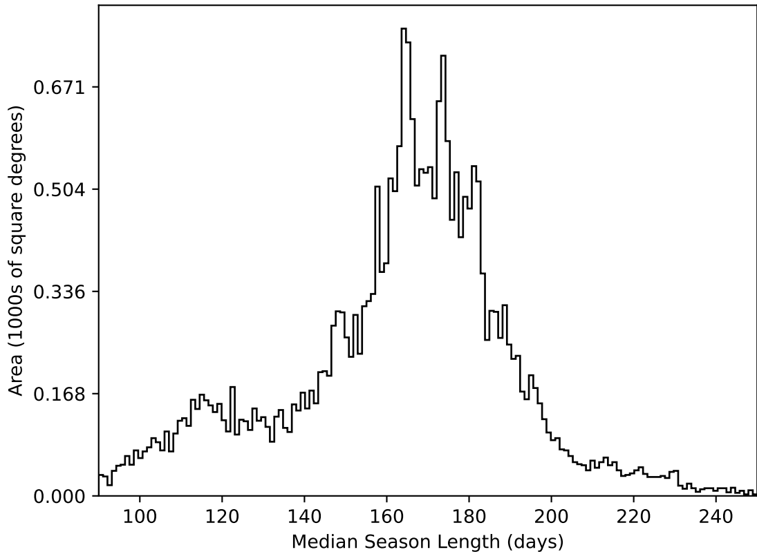
ddf_acor_sf15_lsf30_lsr20_v3.4_10yrs All sky all bands: Median Season Length
