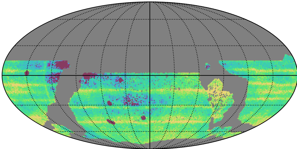
ddf_acor_sf15_lsf30_lsr20_v3.4_10yrs WFD: Median Intra-Night Gap
