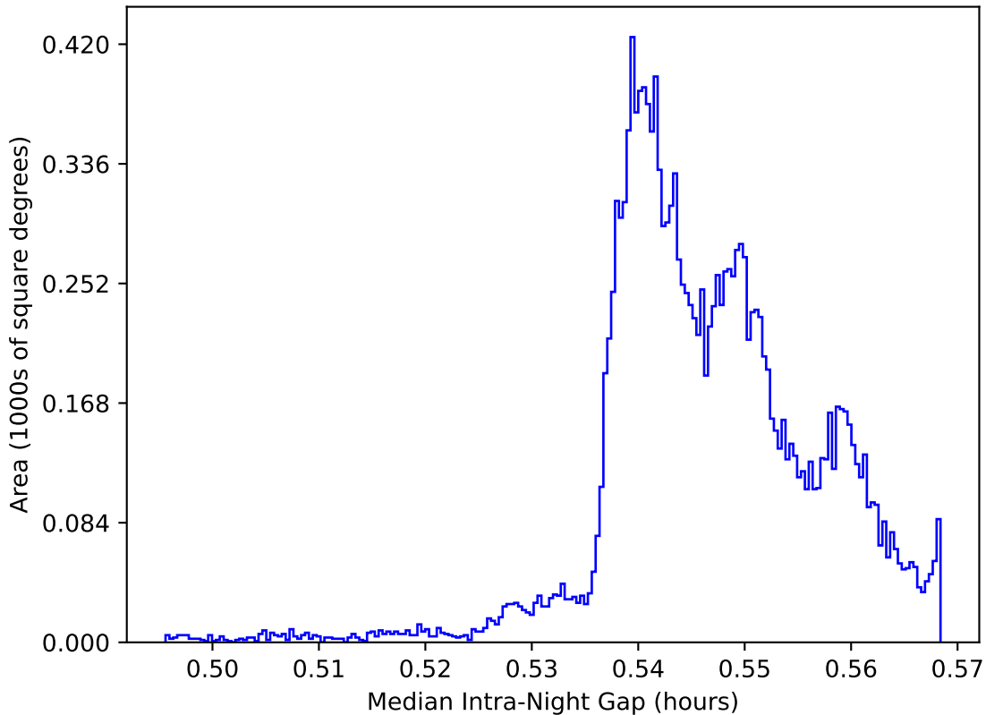
ddf_acor_sf15_lsf30_lsr20_v3.4_10yrs WFD: Median Intra-Night Gap
