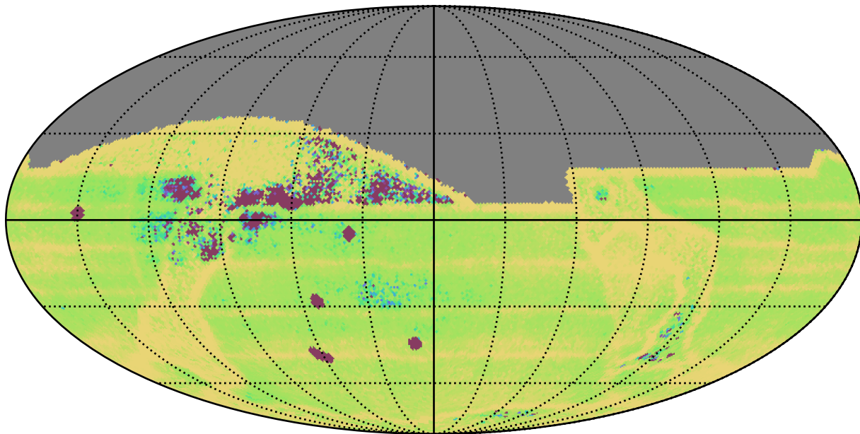
ddf_acor_sf15_lsf30_lsr20_v3.4_10yrs All sky: Median Intra-Night Gap
