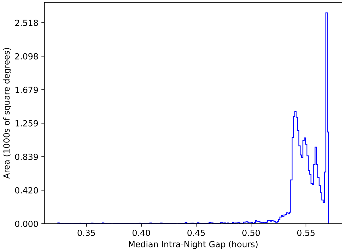
ddf_acor_sf15_lsf30_lsr20_v3.4_10yrs All sky: Median Intra-Night Gap
