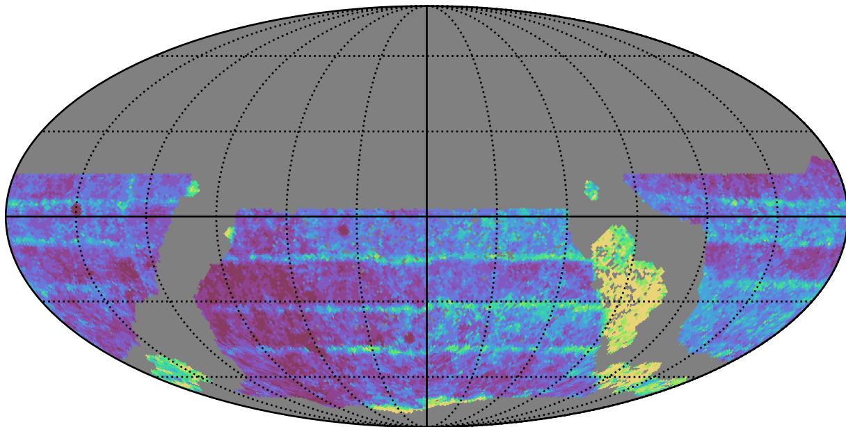
ddf_acor_sf15_lsf30_lsr20_v3.4_10yrs WFD z band: Median Inter-Night Gap
