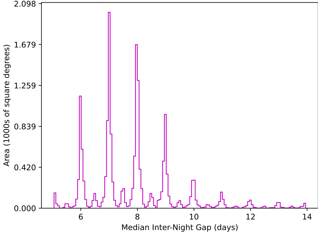
ddf_acor_sf15_lsf30_lsr20_v3.4_10yrs WFD z band: Median Inter-Night Gap
