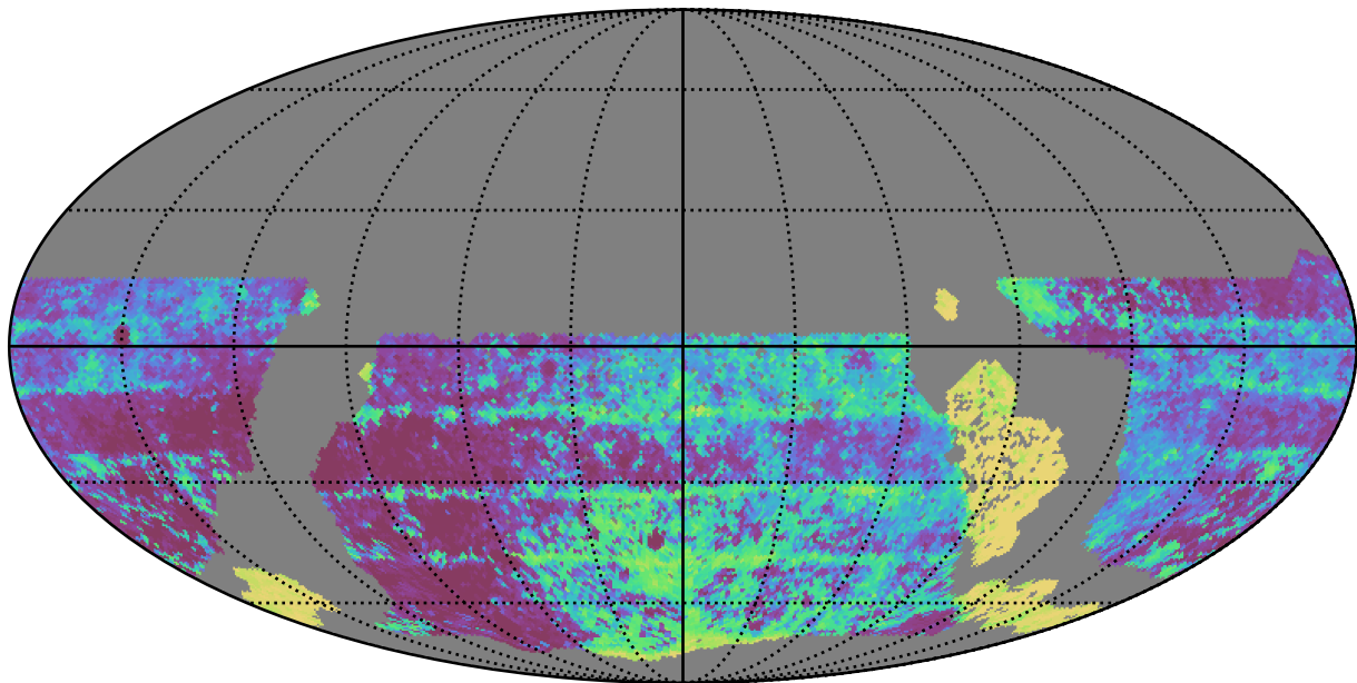
ddf_acor_sf15_lsf30_lsr20_v3.4_10yrs WFD y band: Median Inter-Night Gap
